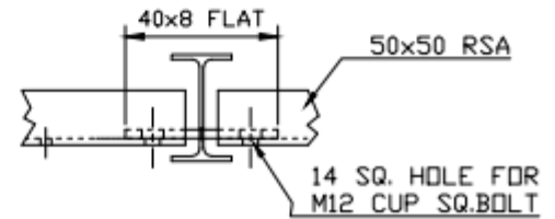
SECTION THRO. POST
