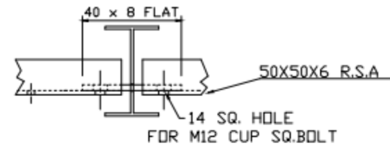
SECTION THRO. POST
