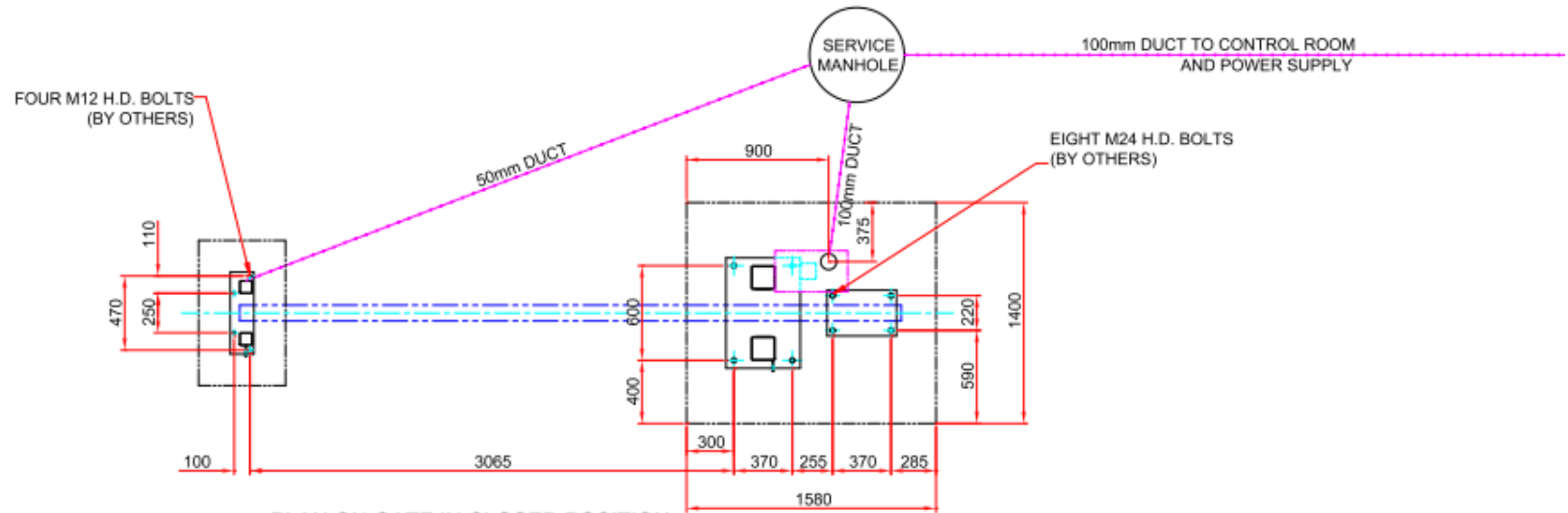
PLAN ON GATE IN CLOSED POSITION
