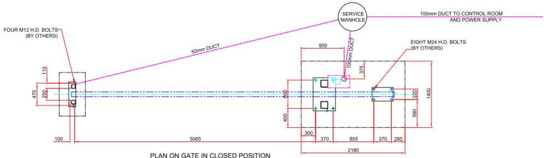
PLAN ON GATE IN CLOSED POSITION
