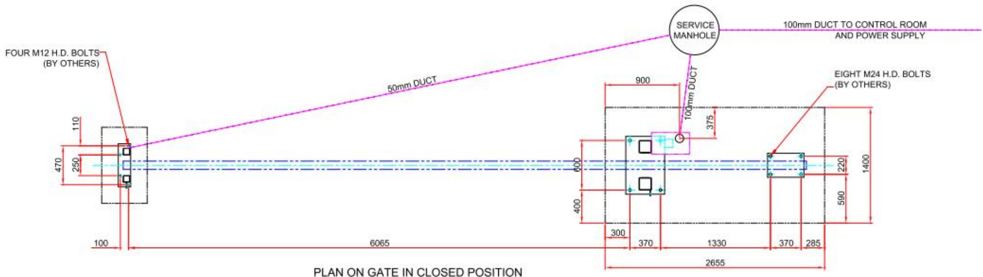
PLAN ON GATE IN CLOSED POSITION
